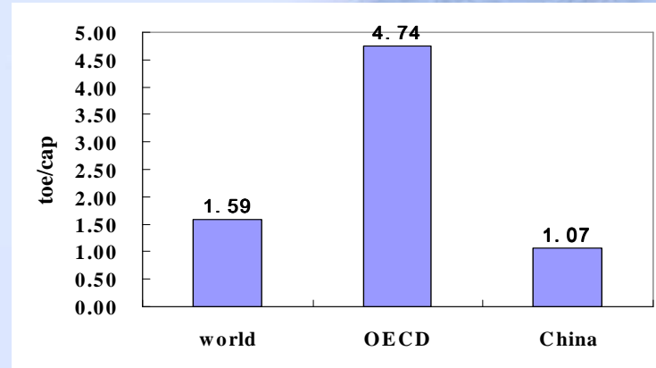
Per capita energy consumption
